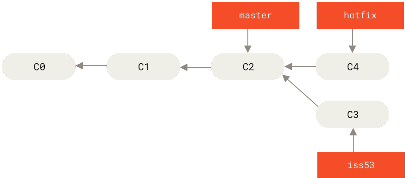
Figure 21. Hotfix branch based on master
