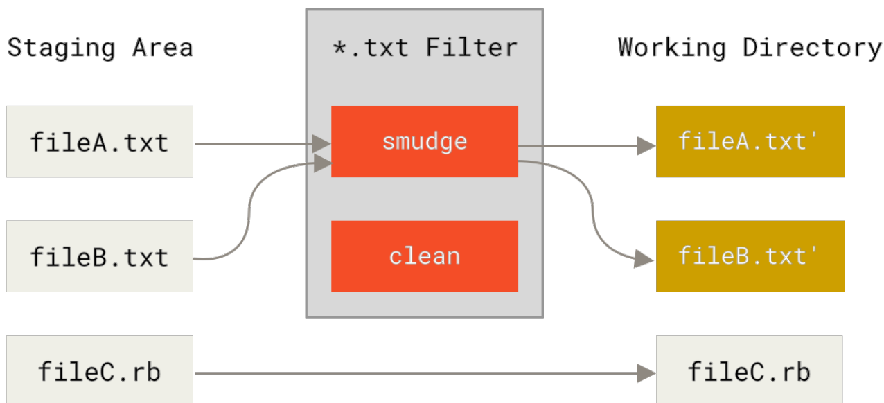
Figure 143. The “smudge” filter is run on checkout
